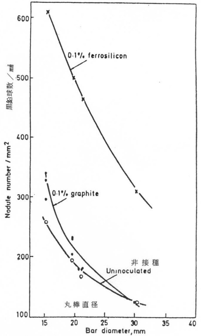
Fig. 1 Relation between nodule number and bar diameter for irons inoculated in the metal stream with graphite and ferrosilicon inoculants.
